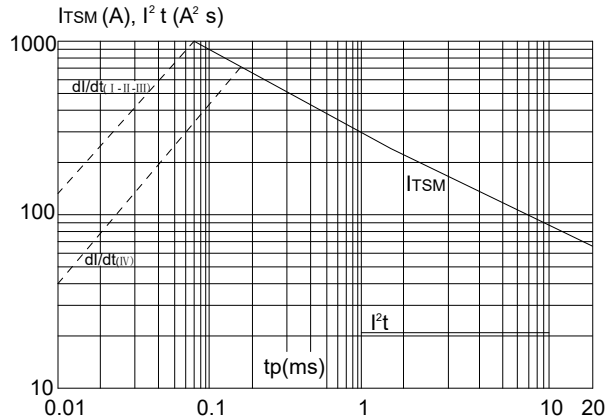
FIG.5: Non-repetitive surge peak on-state current for a sinusoidal pulse with width t_p < 20\text{ms} , and corresponding value of \int I^2 t (I - II - III: dI/dt < 50\text{A}/\mu\text{s} ; IV: dI/dt < 10\text{A}/\mu\text{s} )
